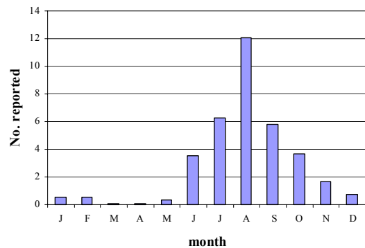
Figure 13. All leatherbacks average over 1994-2004.
